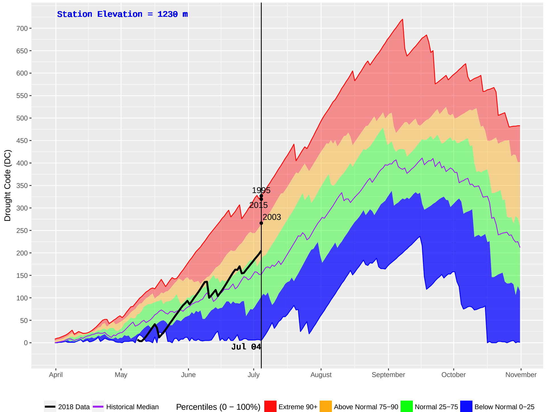
SLOCAN (406) : Historical (1992–2016) and Current (2018) Noon Drought Code (DC)
