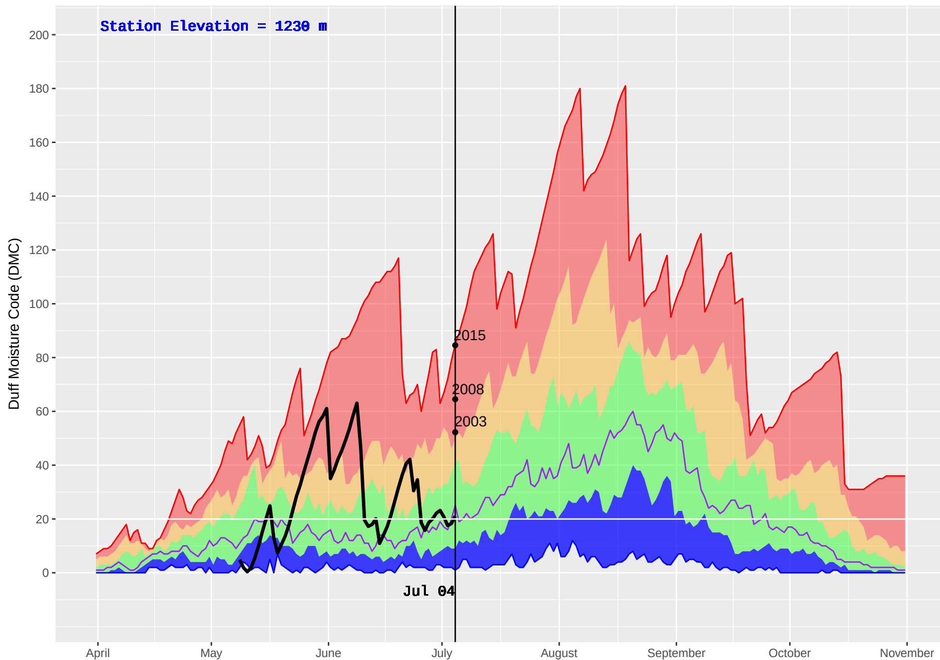
SLOCAN (406) : Historical (1992–2016) and Current (2018) Noon Duff Moisture Code (DMC)
