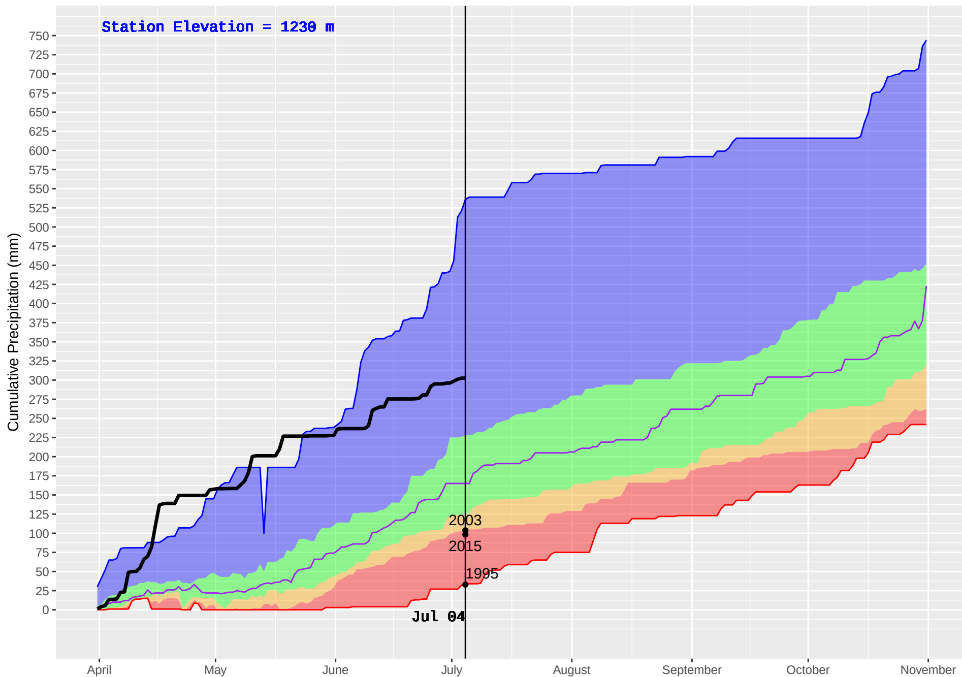
SLOCAN (406) : Historical (1992–2016) and Current (2018) Noon Cumulative Precipitation
